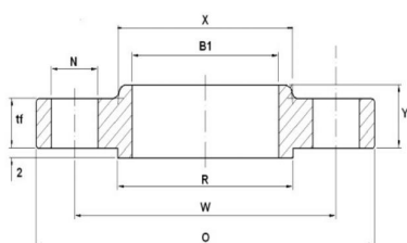
SO Slip-on
