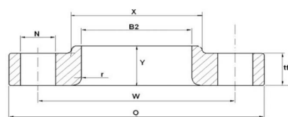
SOLTO Lapped
